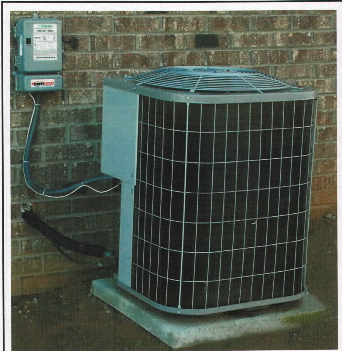
Typical Load Control Switch Install – With Comserve Direct Control Unit Shown (Actual Switch Manufacturer to be Determined)
