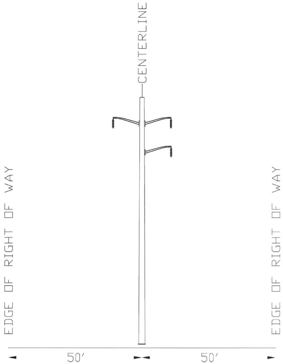
TYPICAL RIGHT-OF-WAY CROSS SECTION
