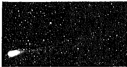
Comet O/1996 B2, better known as Comet Hyakutake, was a spectacular sight in the evening sky. In 1996, its tail stretched across several constellations.
