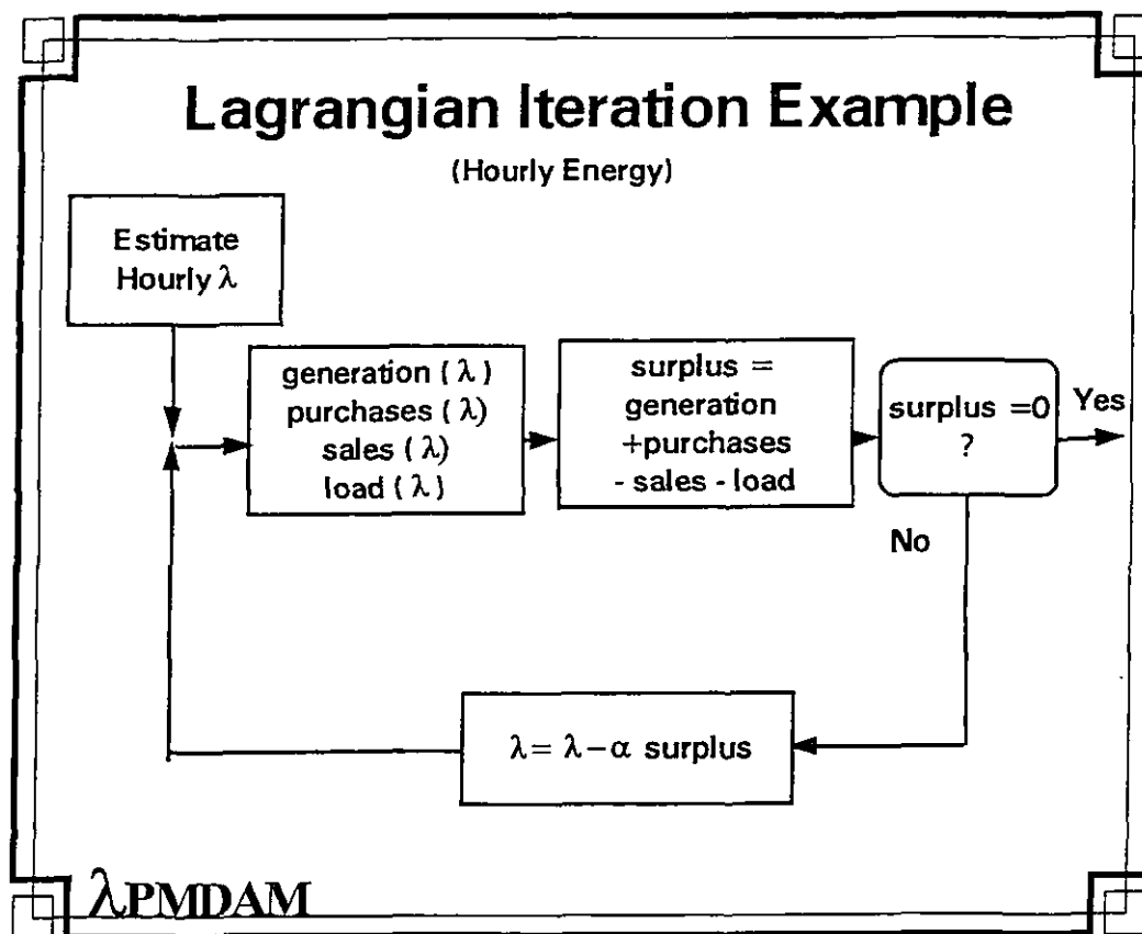
Figure 2 Lagrangian Iteration
