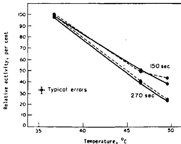
Fig. 3.6. Relative activity of yeast glucose-6-phosphate dehydrogenase as a function of temperature: - - -, treatment with microwave radiation; —, treatment without microwave radiation. Upper lines, 150-s treatment; lower lines, 270-s treatment. (From Belkhode et al. , 1974b.)
