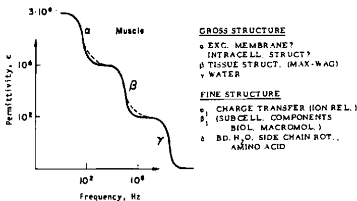
Fig. 2.2. Gross and fine structural relaxation contributions to the dielectric constant of muscle tissue. Dashed lines indicate fine structural contributions. The data and various structural contributions are typical for all tissues of high water content. (From Schwan, 1976.)
