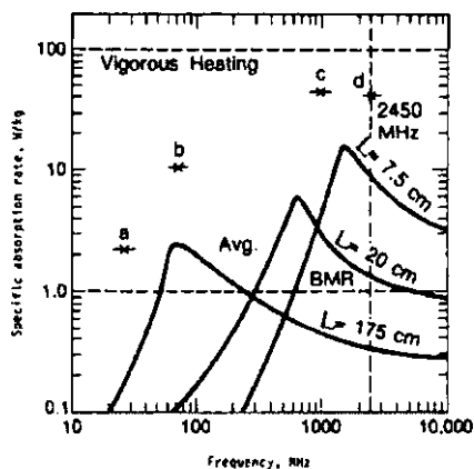
Fig. 17.1. Average SAR measured in prolate spheroids of various lengths, L , for an exposure to a power density at 10 \text{ mW/cm}^2 at various frequencies. These models are used to simulate exposure of various experimental subjects in RFEM fields (after Gandhi, 1979). The points identified by the letters a, b, c and d indicate maximal localized SAR levels based on measurements as follows: a and b, in models of human beings (Guy et al. , 1978, 1983); c, in rats (Lin et al. , 1977); and d, in mice (Chou and Guy, 1982.) The average basal metabolic rate (BMR) is shown by the lower dashed horizontal line.
