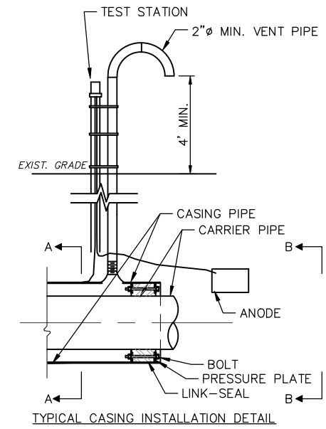
TYPICAL CASING INSTALLATION DETAIL
