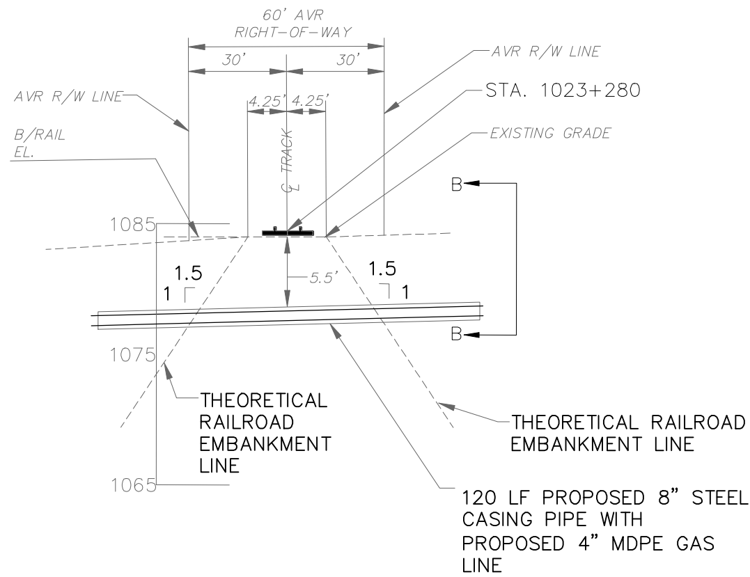
PROFILE VIEW A-A
