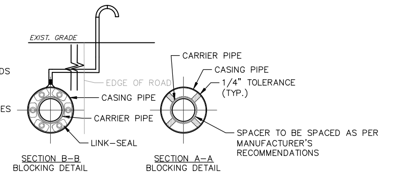
TYPICAL CASING INSTALLATION DETAIL
