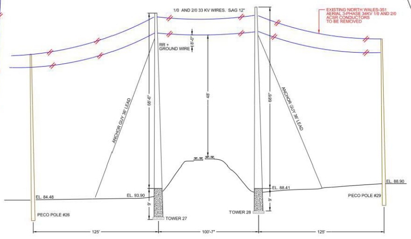
ELEVATION SCALE: HORIZONTAL: 1:50 VERTICAL: 1:20
