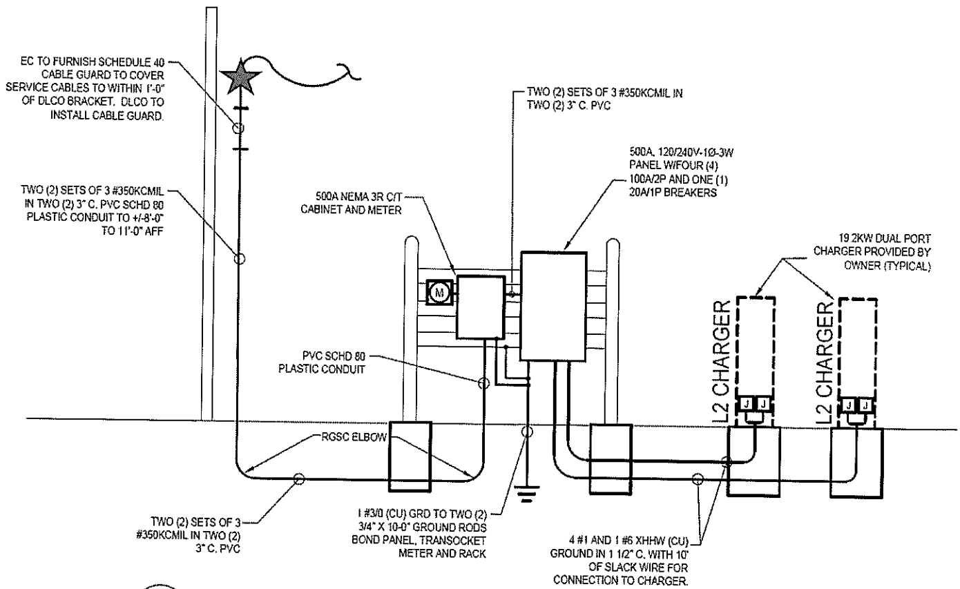
2 POWER RISER DIAGRAM - 120/240V, 1P, 3W E-1 NO SCALE
