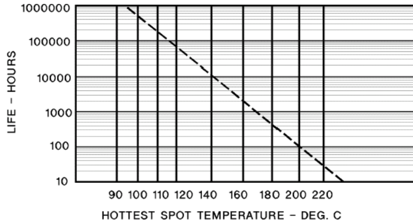
Figure 3—Minimum life expectancy curve for liquid-immersed distribution, power, and regulating transformers rated in accordance with Clause 5, at 65 °C average winding rise, 80 °C hottest-spot rise
