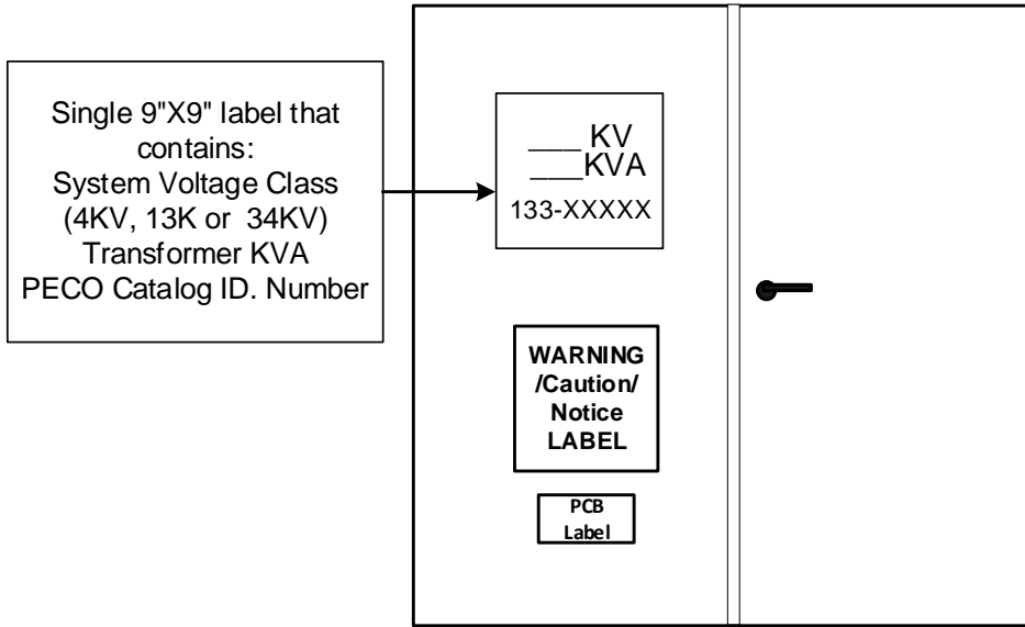
TRANSFORMER FRONT VIEW
