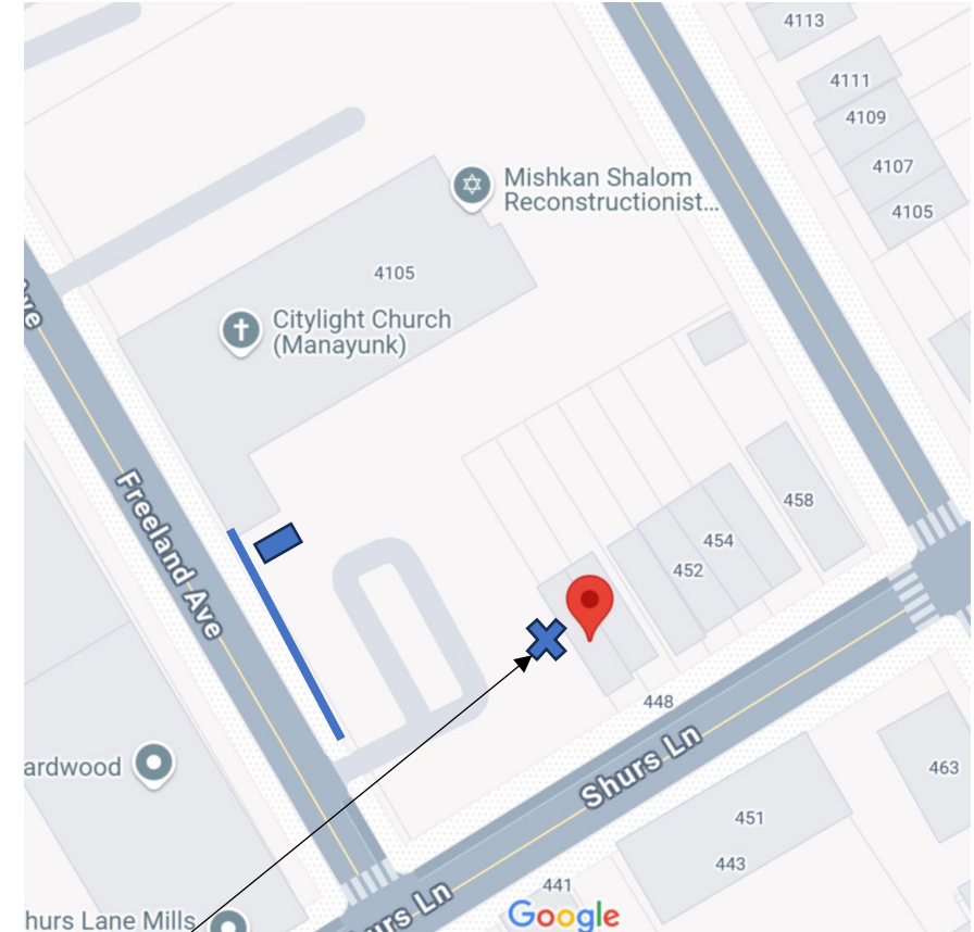
53.7 dB at approx. 65 ft from transformer in parking lot midway down the house line
