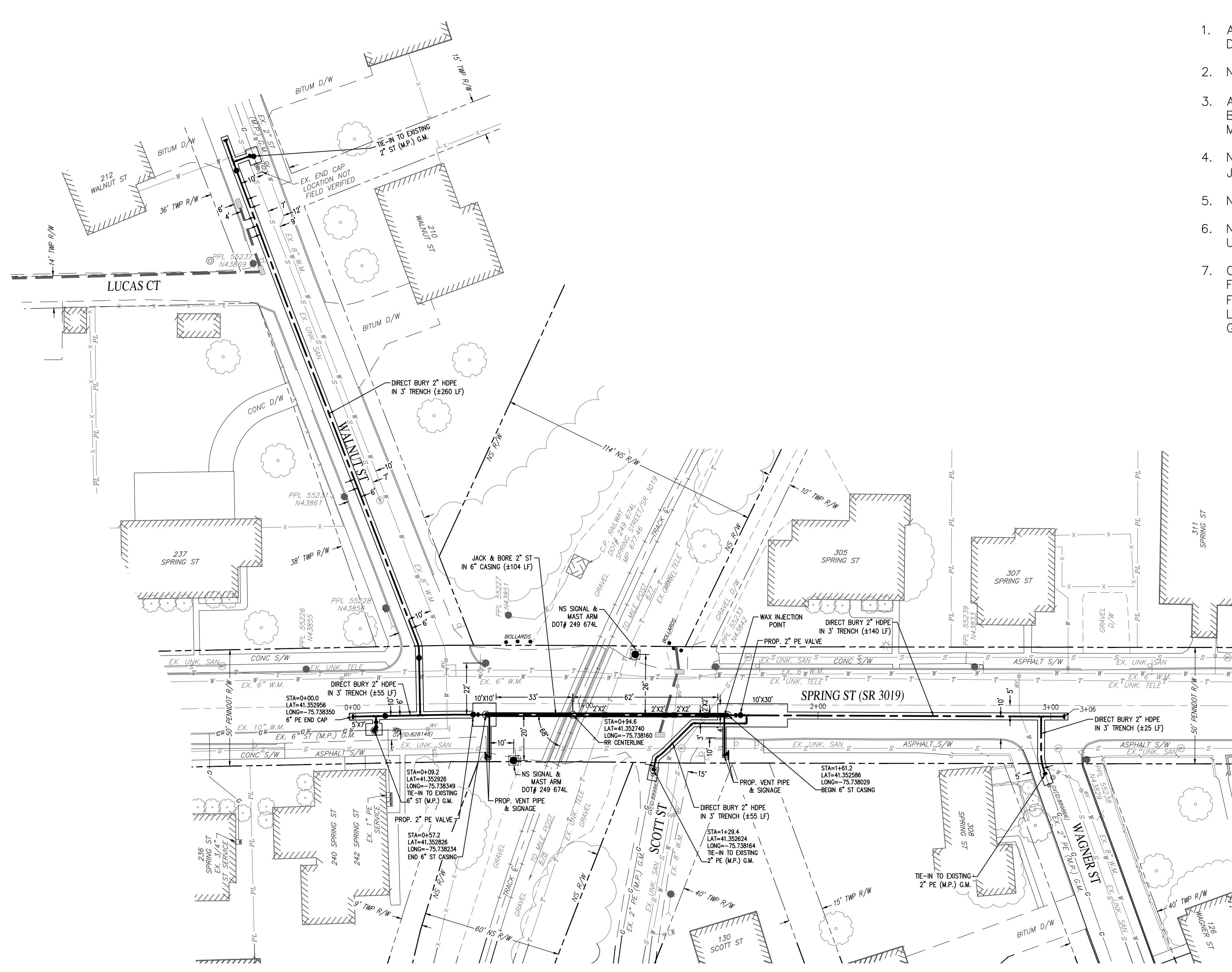
PLAN VIEW (HORIZONTAL SCALE 1"=10')
